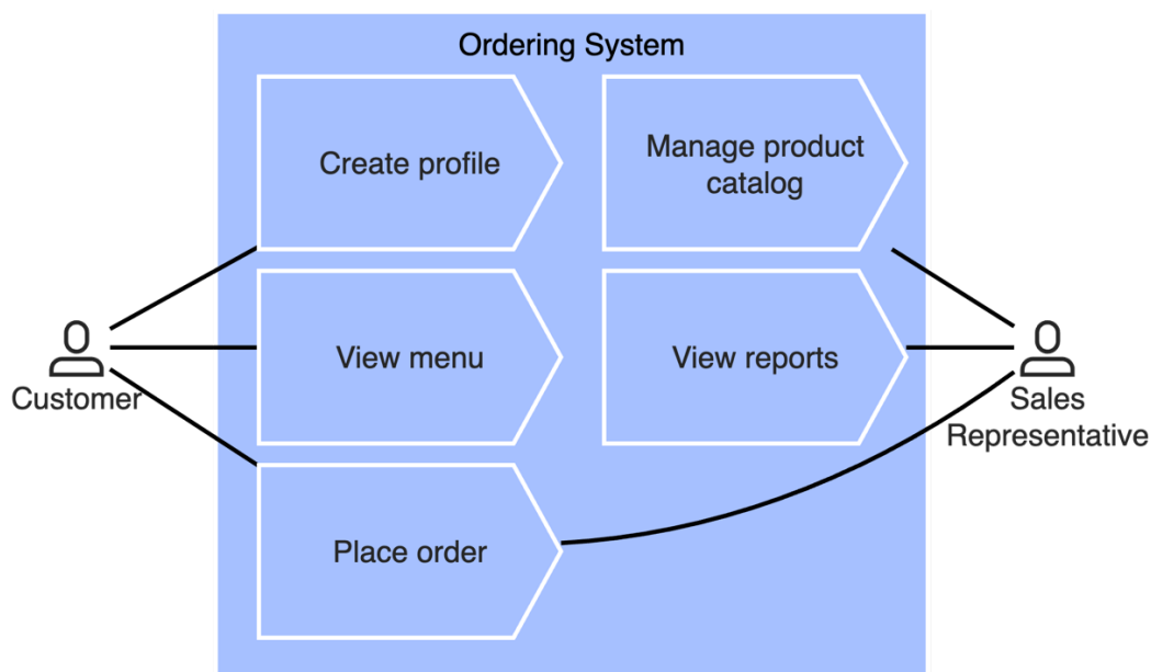
Figure 99: Process -elements as internal functionalities of an application.
