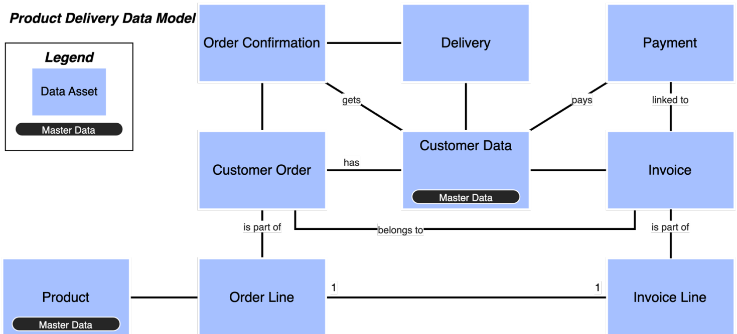
Figure 241: Data model - assets as data elements / -objects.
