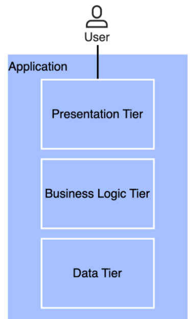
Figure 256: Three-tiered architecture.
