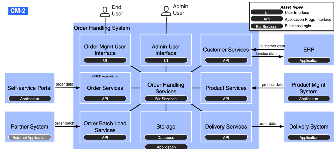
Figure 276: CM-2 composition diagram.
