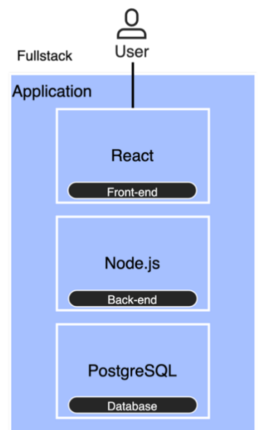
Figure 257: Full stack example with typed assets.
