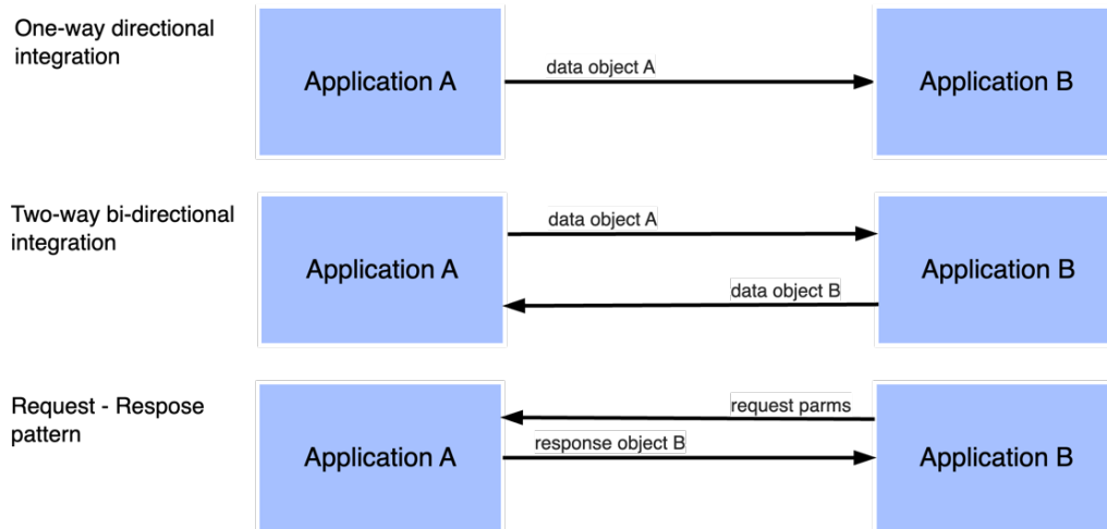
Figure 290: Application integration patterns.
