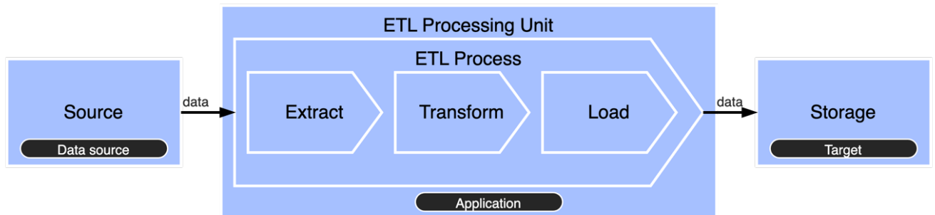
Figure 261: Extract-Transform-Load pattern.
