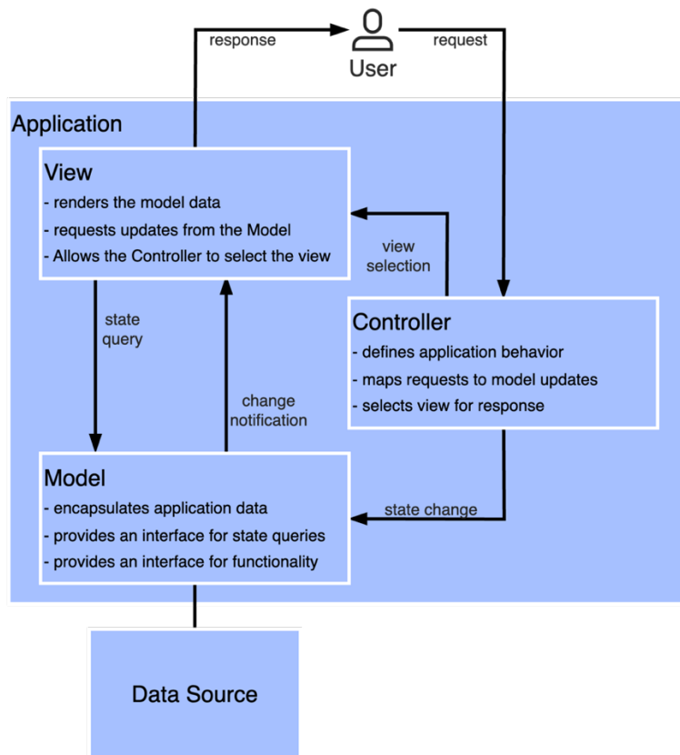
Figure 259: Model-View-Controller (MVC) pattern.
