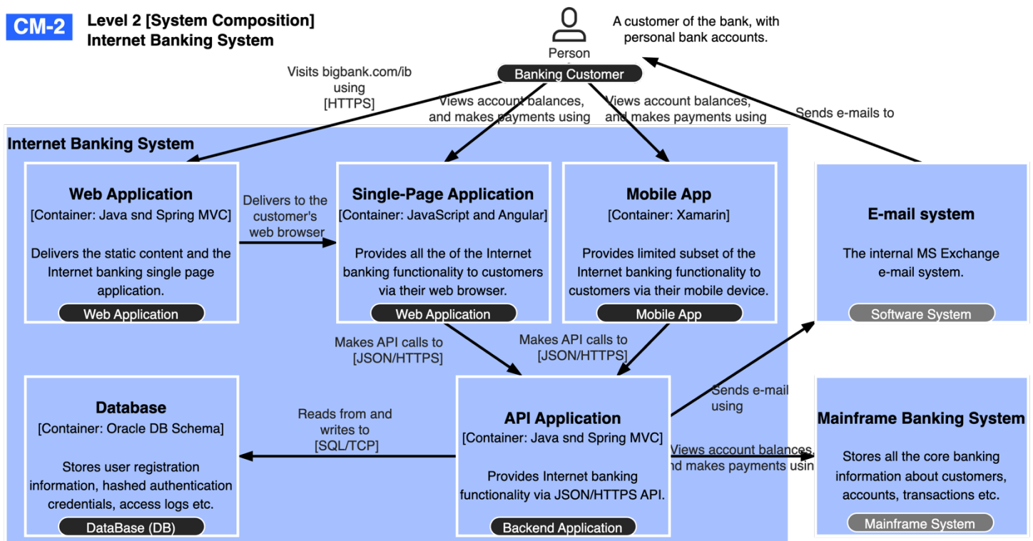
Figure 281: CM-2 Application architecture at a detailed level, the internal structure.
