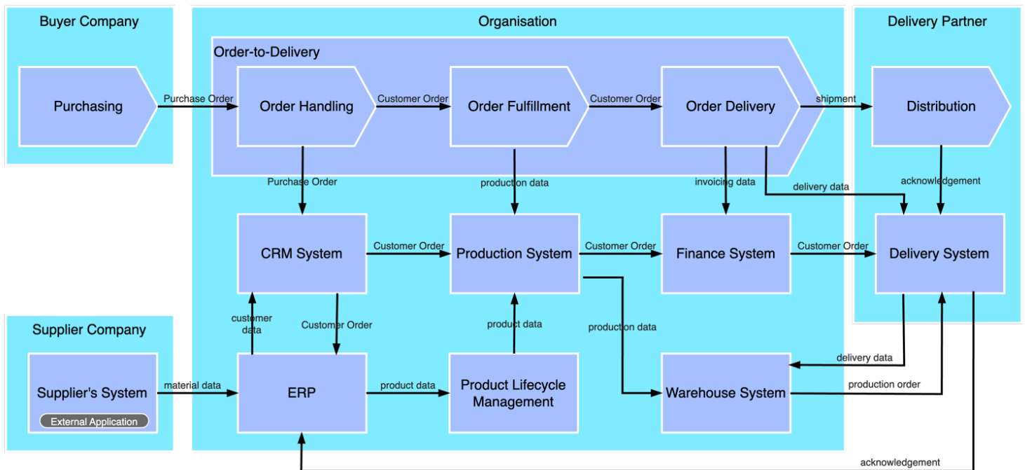
Figure 248: Data flows between the processes and applications in a B2B scenario.
