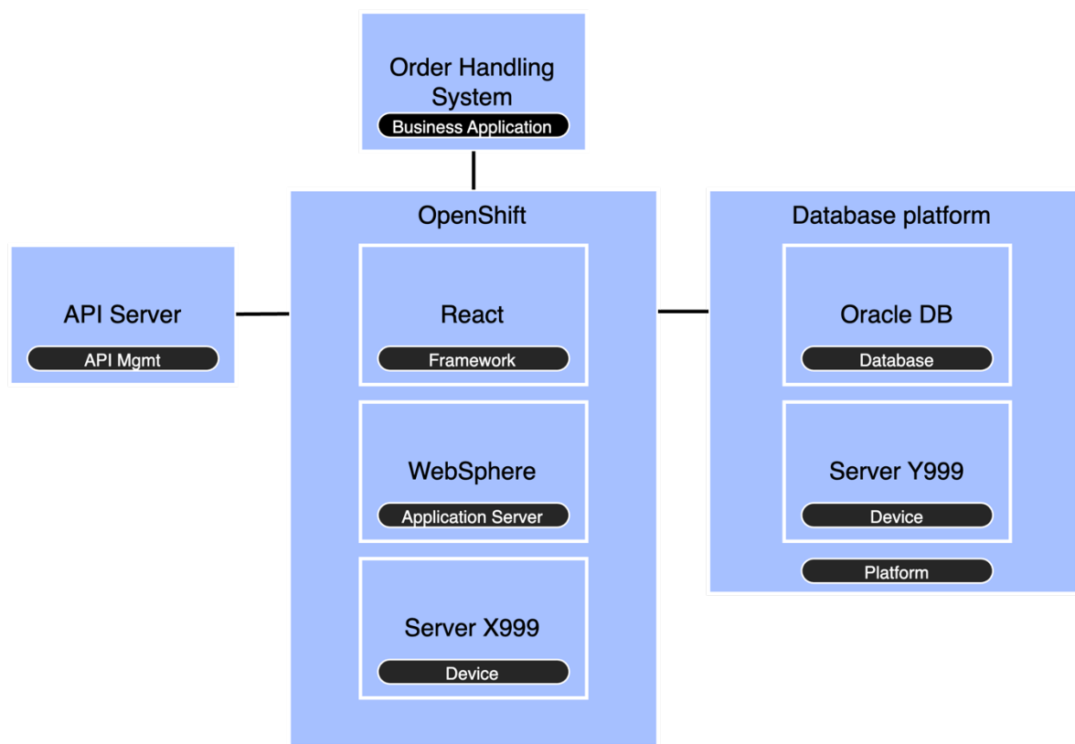
Figure 283: Deployment diagram.
