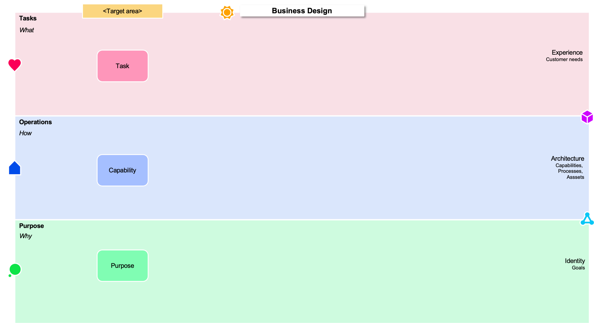
Figure 594: What-How-Why.
