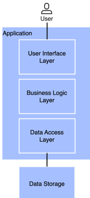
Figure 258: Layered Architecture.
